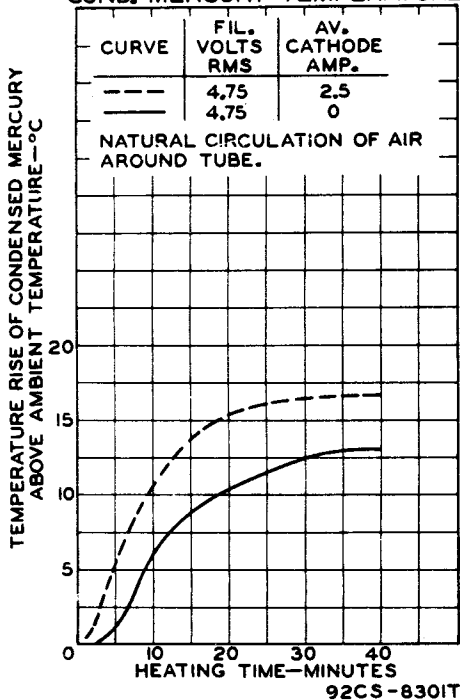
RATE OF RISE OF COND.-MERCURY TEMPERATURE
